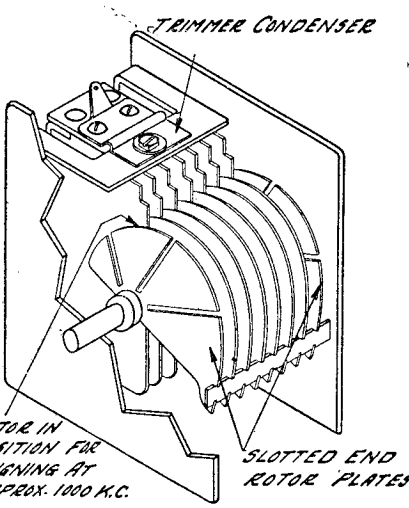
Condenser Section with Shield Plate Cut Away
